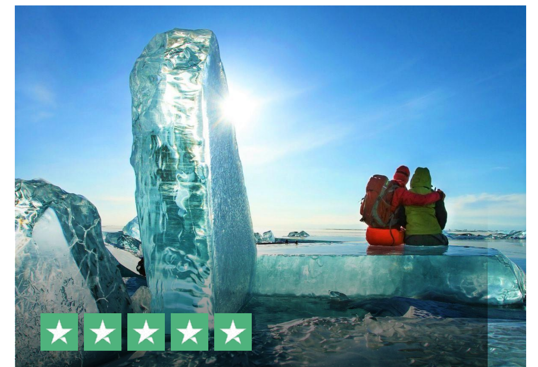
Crystal Ice of Lake Baikal
